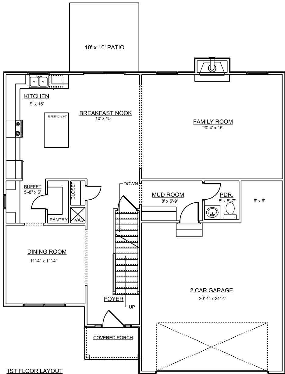
1ST FLOOR LAYOUT
