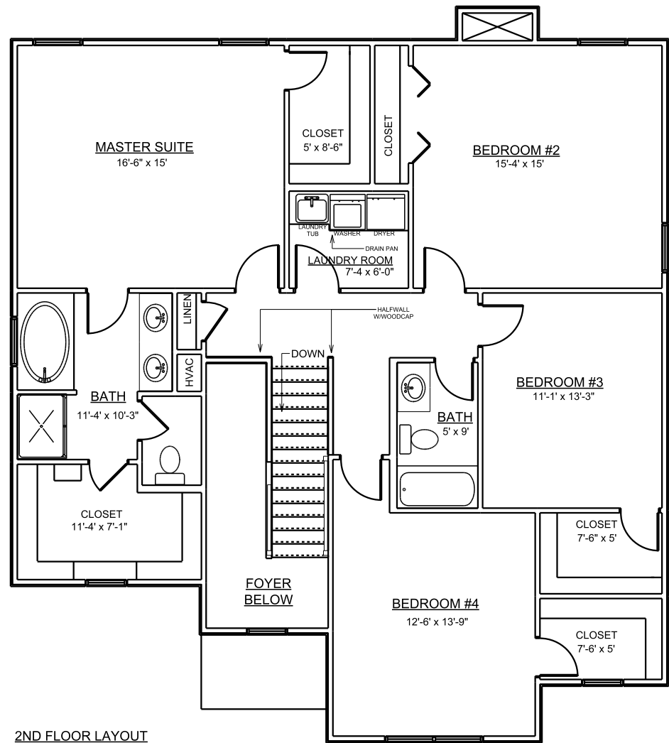
2ND FLOOR LAYOUT
